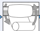
Wrap the Fiberglass tape around the repair area as tightly and evenly as possible using the entire roll
